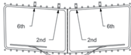
[1988 & 2005] Flat Top Factory Bracket Locations
